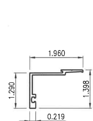
13 SUN-4071 FACE CAP 1-5/16" GLAZING
