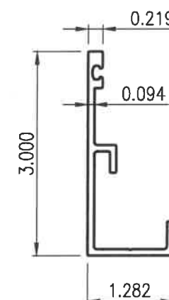
8 SUN-403 FACE CAP 9/16" GLAZING
