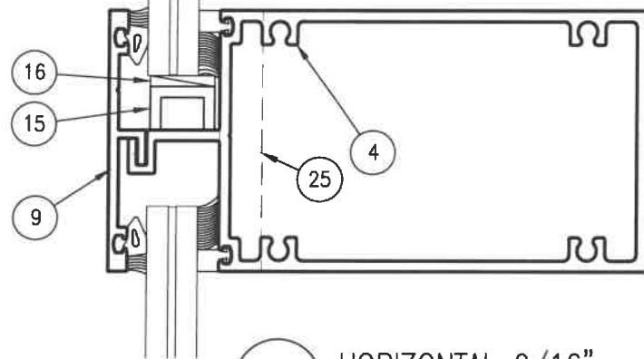
2 HORIZONTAL 9/16" Glazing condition G3 Glazing condition G1 similar (Ref SHT 8 of 8) Scale: 6" = 1'-0"
