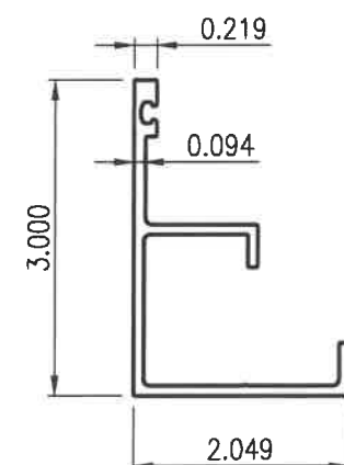
11 SUN-436 FACE CAP 1-5/16" GLAZING
