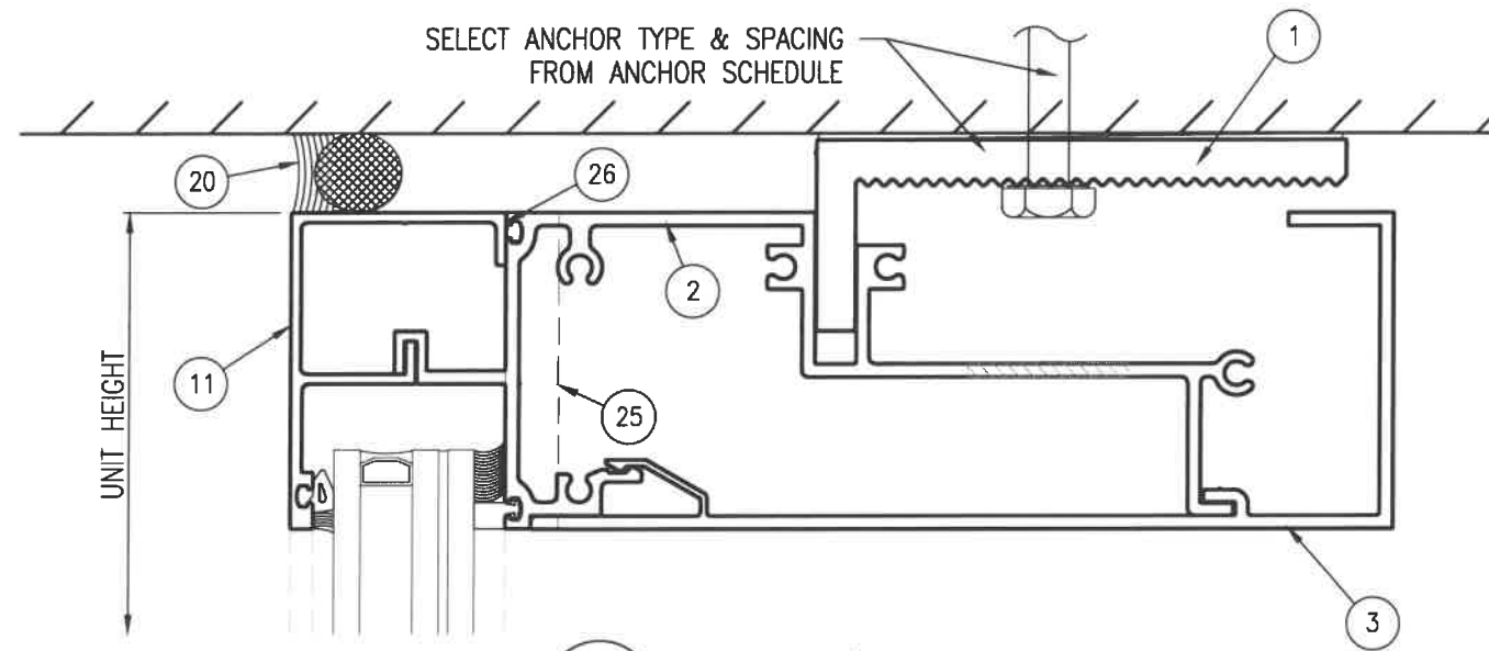
6 HEAD 1 5/16" Glazing condition G4 Glazing condition G2 similar (Ref SHT 8 of 8) Scale: 6" = 1'-0"
