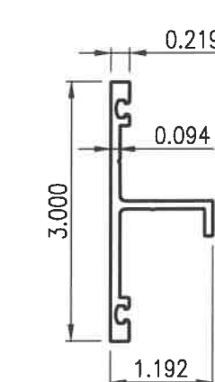
12 SUN-437 FACE CAP 1-5/16" GLAZING
