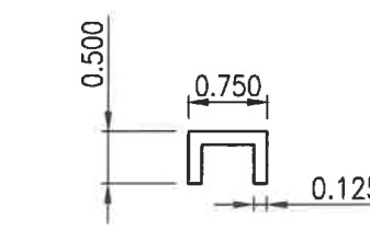
15 SETTING CHAIR 3/4"x1/2"x1/8" CHANNEL
