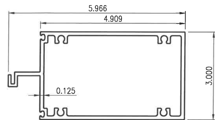
4 SUN-605 HORIZONTAL
