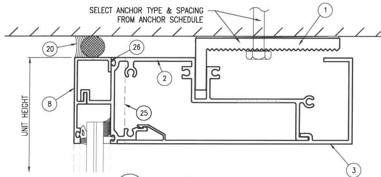
3 HEAD 9/16" Glazing condition G3 Glazing condition G1 similar (Ref SHT 8 of 8) Scale: 6" = 1'-0"
