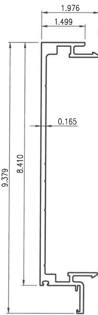
6 SUN-1009 SPLIT MULL MALE
