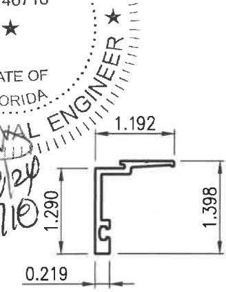
10 SUN-4070 FACE CAP 9/16" GLAZING
