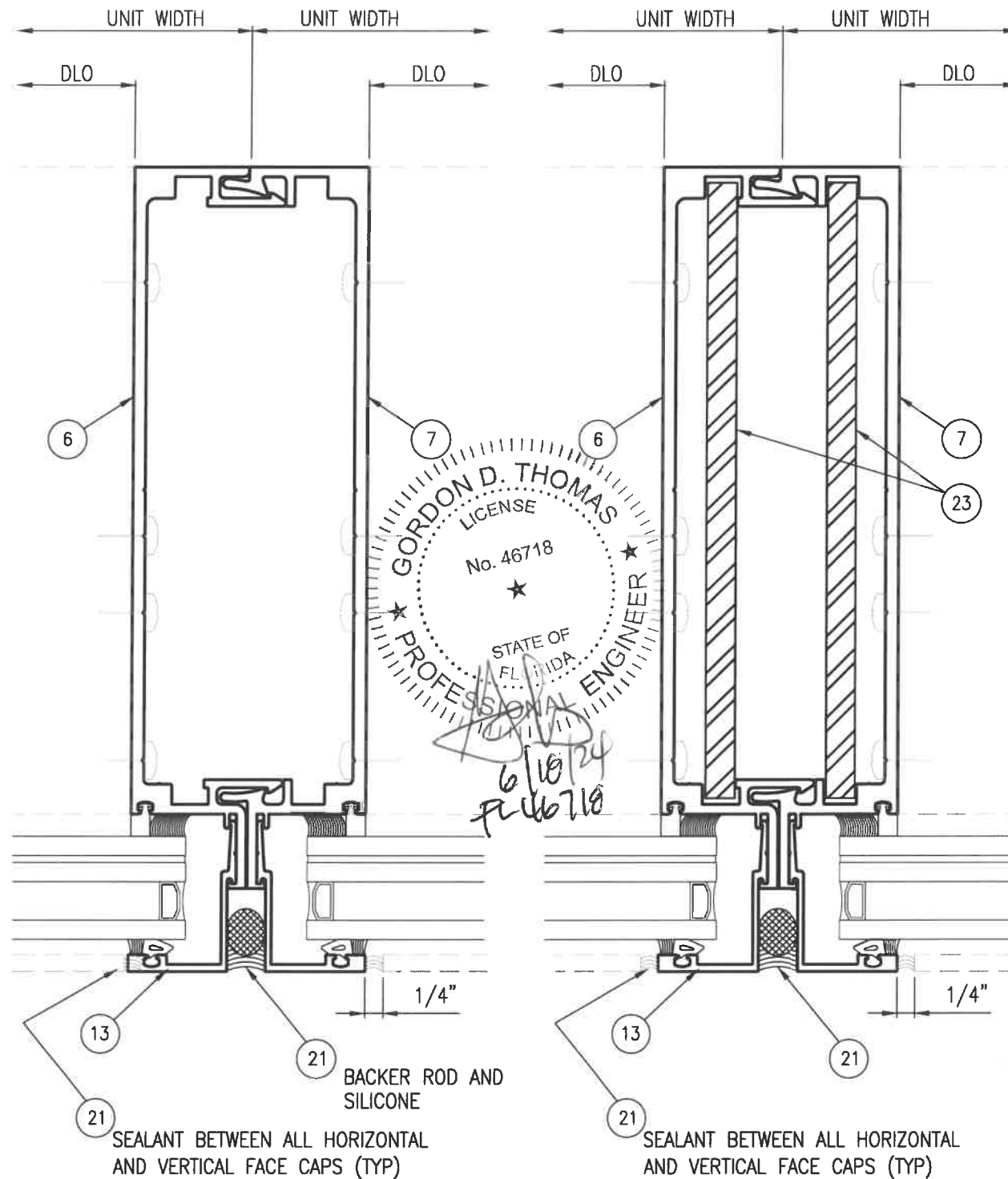
2 UNREINFORCED MULLION Glazing condition G4 Scale: 6" = 1'-0" Glazing condition G2 similar (Ref SHT 8 of 8)
