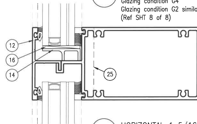
5 HORIZONTAL 1 5/16" Glazing condition G4 Glazing condition G2 similar (Ref SHT 8 of 8) Scale: 6" = 1'-0"
