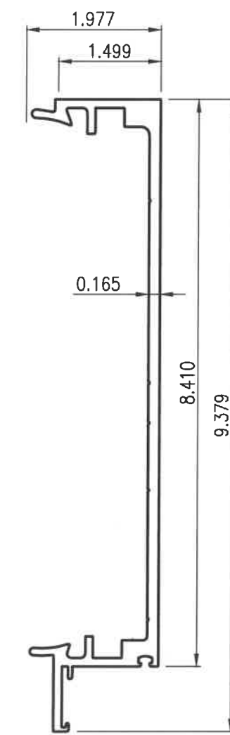
7 SUN-1010 SPLIT MULL FEMALE
